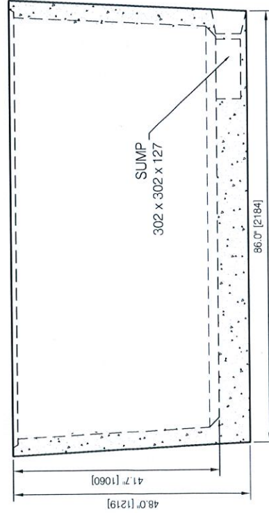
ELEVATION VIEW
