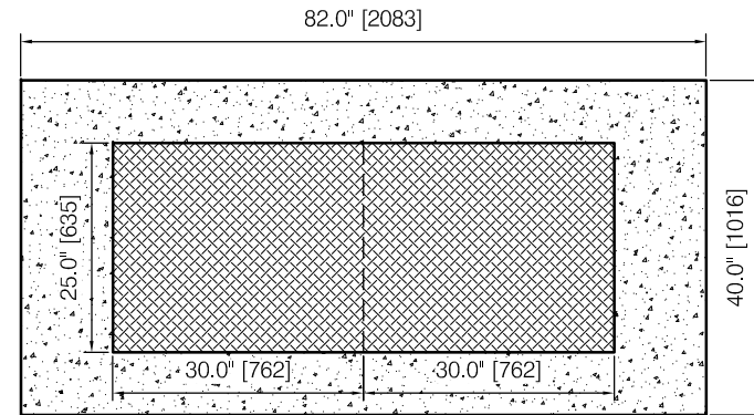
TYPE 2 - for 2 manhole casting
