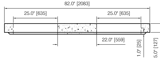
TYPE 2 - for 2 manhole casting
