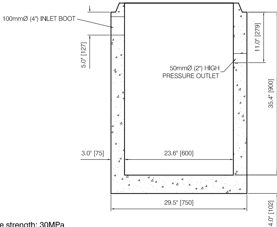
Section View
