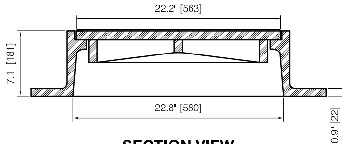
SECTION VIEW
