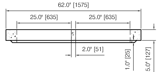
TYPE 2 - for 2 manhole casting
