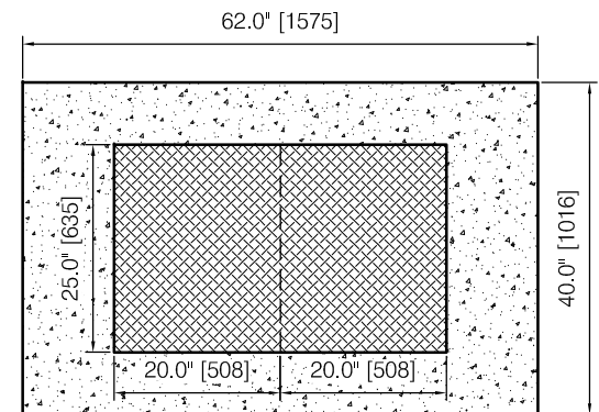
TYPE 2 - for 2 manhole casting
