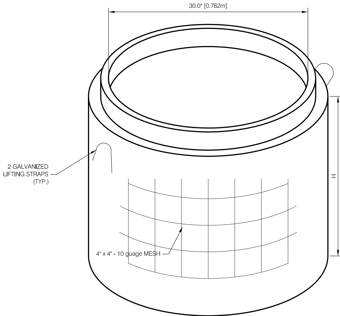
ISOMETRIC VIEW
