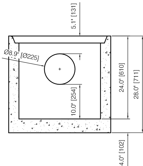
Section View of Lawn Basins
