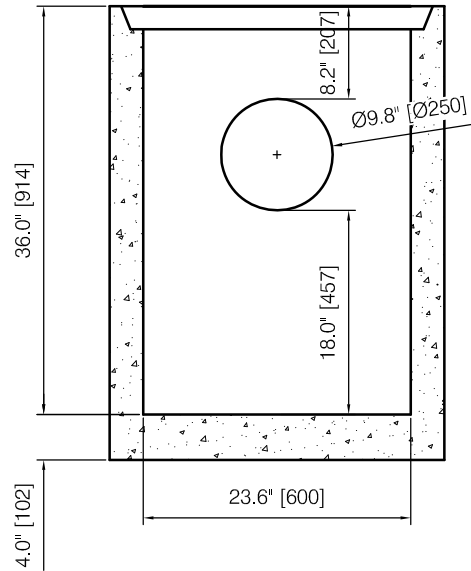
Section View of Lawn Basins
