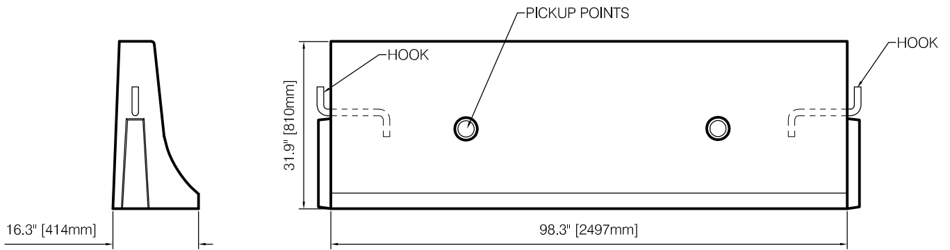
MALE BARRIER
