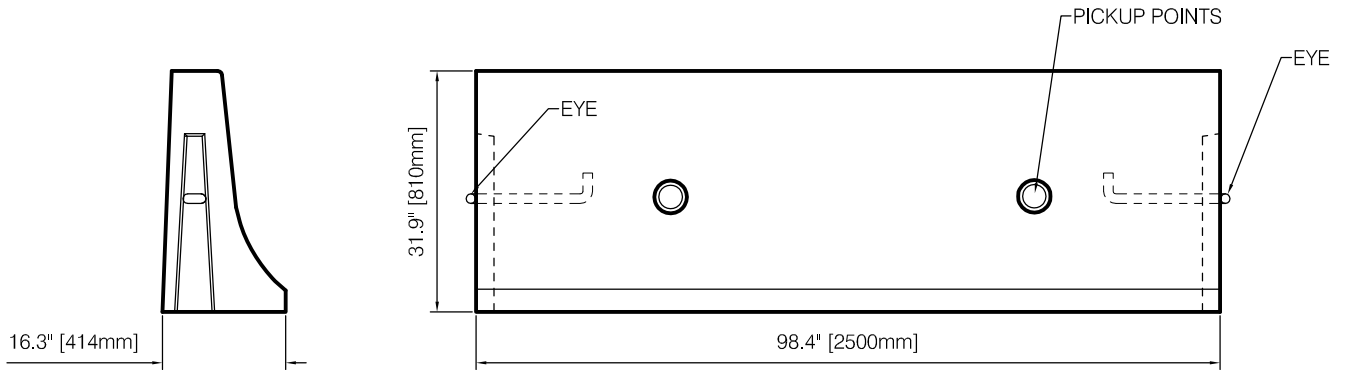
FEMALE BARRIER
