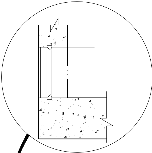
MANHOLE INLET/OUTLET DETAIL
