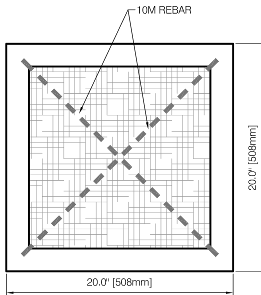
PLAN VIEW
