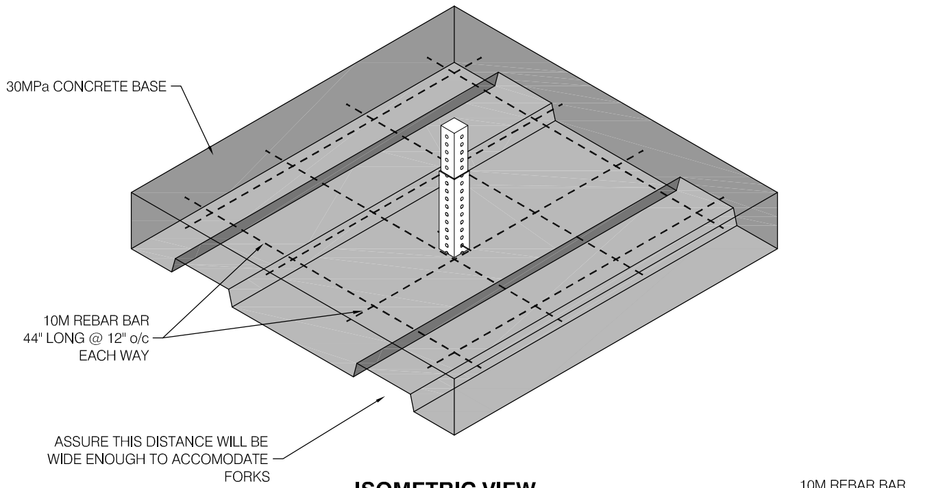
ISOMETRIC VIEW
