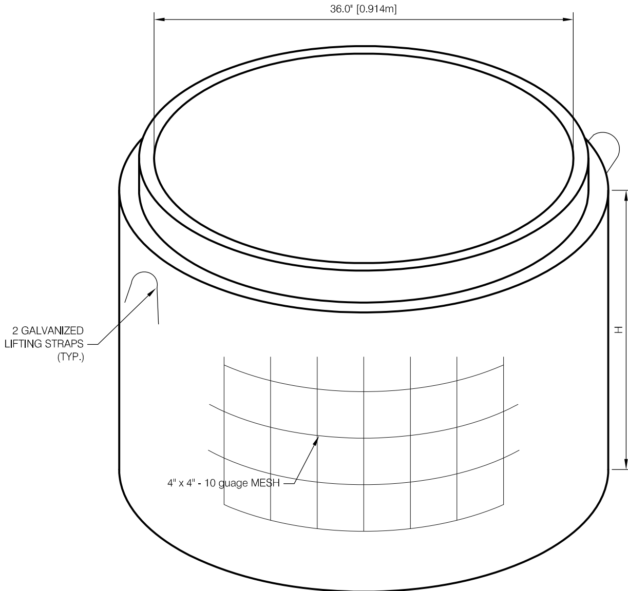
ISOMETRIC VIEW
