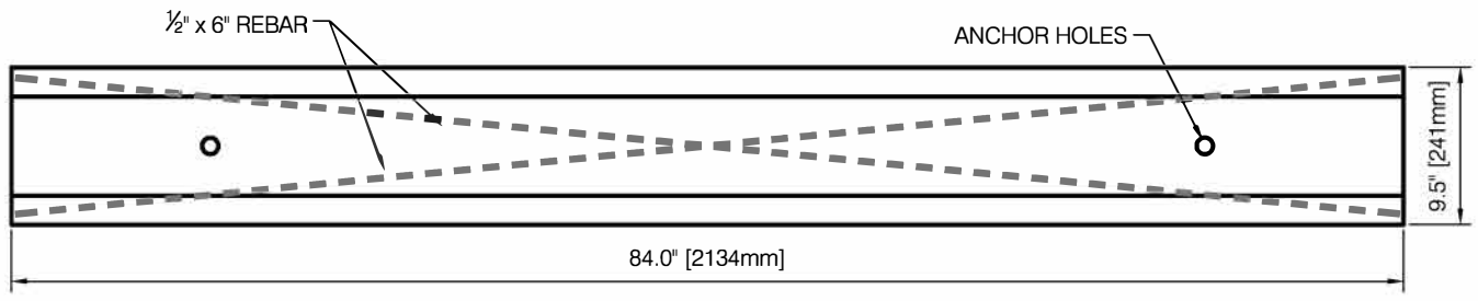
PLAN VIEW
