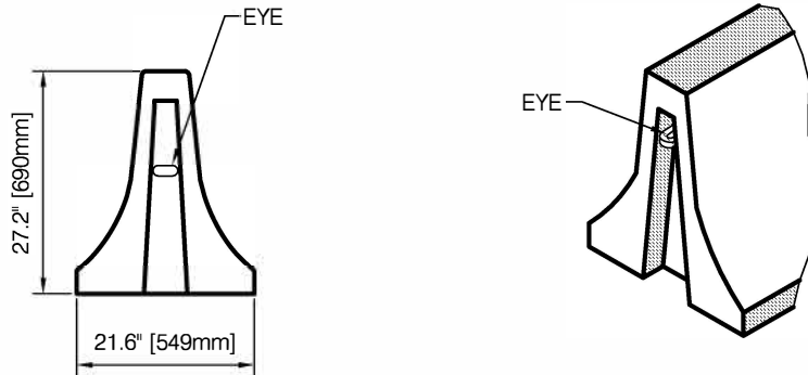
END DETAIL
